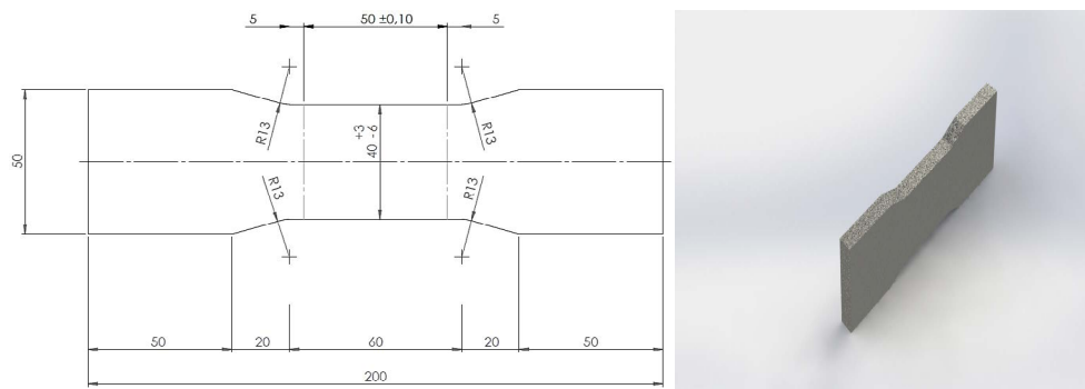
Figure 1. Main dimensions of test specimen.
