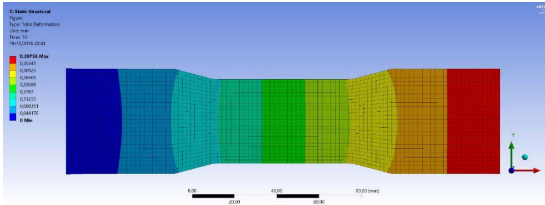
Figure 2. Total deformation of CDP through static structure analysis.
